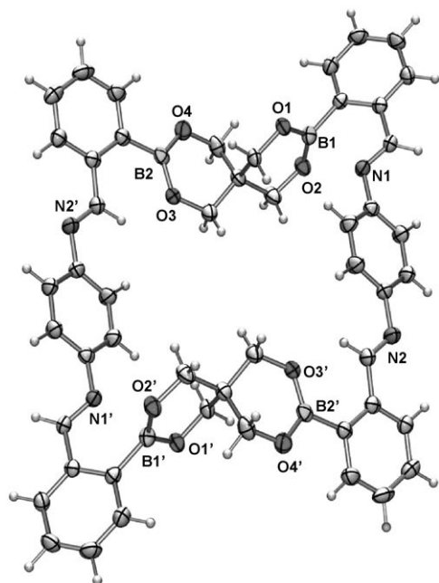
Figure 1. Crystal structure of centrosymmetric macrocycle 16 2D .
